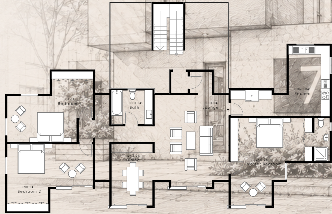
Second Floor Layout
